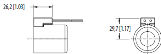
W0 Leadwire
